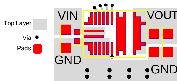
Figure 6: Recommended PCB Layout
