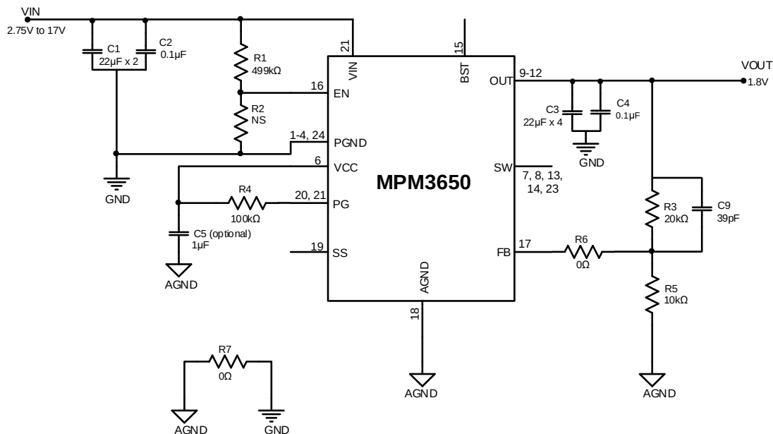
Figure 8: Typical Application Circuits with 1.8V Output
