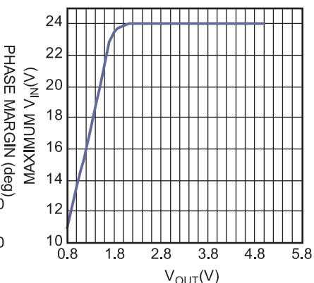
Maximum V_{IN} vs. V_{OUT}
