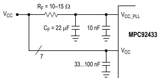
Figure 7. V CC_PLL Power Supply Filter
