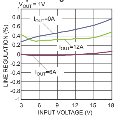
Line Regulation vs. Input Voltage
