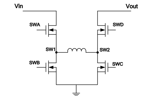
Figure 3: Buck-Boost Topology
