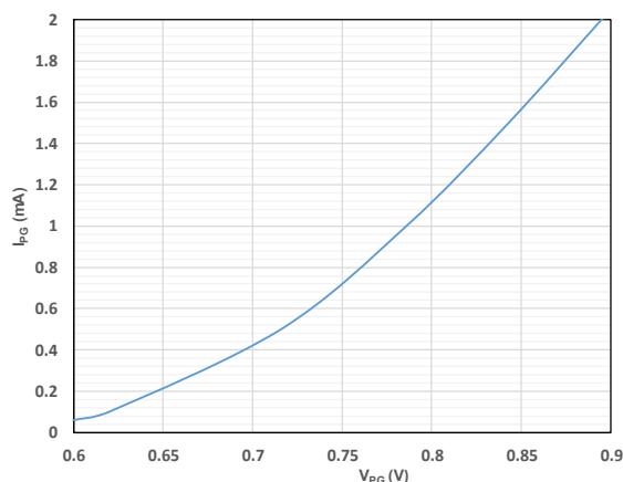
Figure 8: PGOOD Clamped Voltage vs. Pull-Up Current
