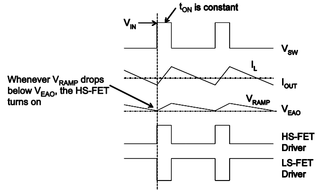
Figure 3: Heavy-Load Operation
