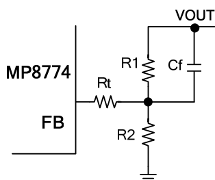
Figure 7: Feedback Network
