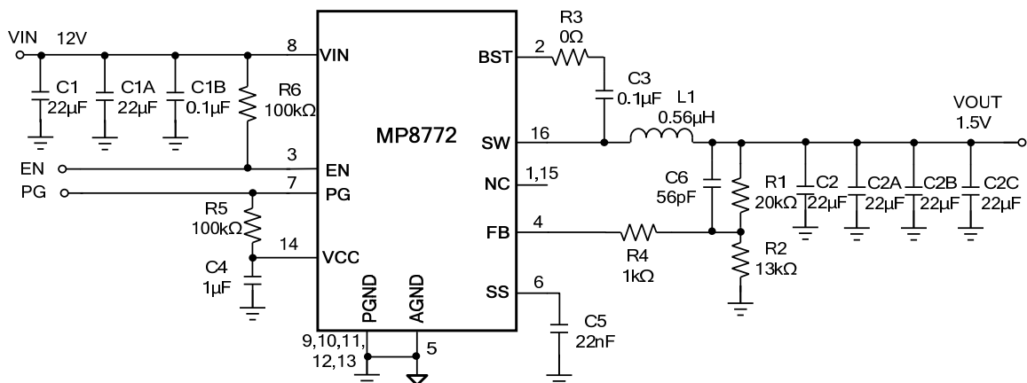
Figure 11: V_{IN} = 12V , V_{OUT} = 1.5V , I_{OUT} = 12A (8)
