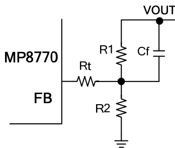
Figure 7: Feedback Network
