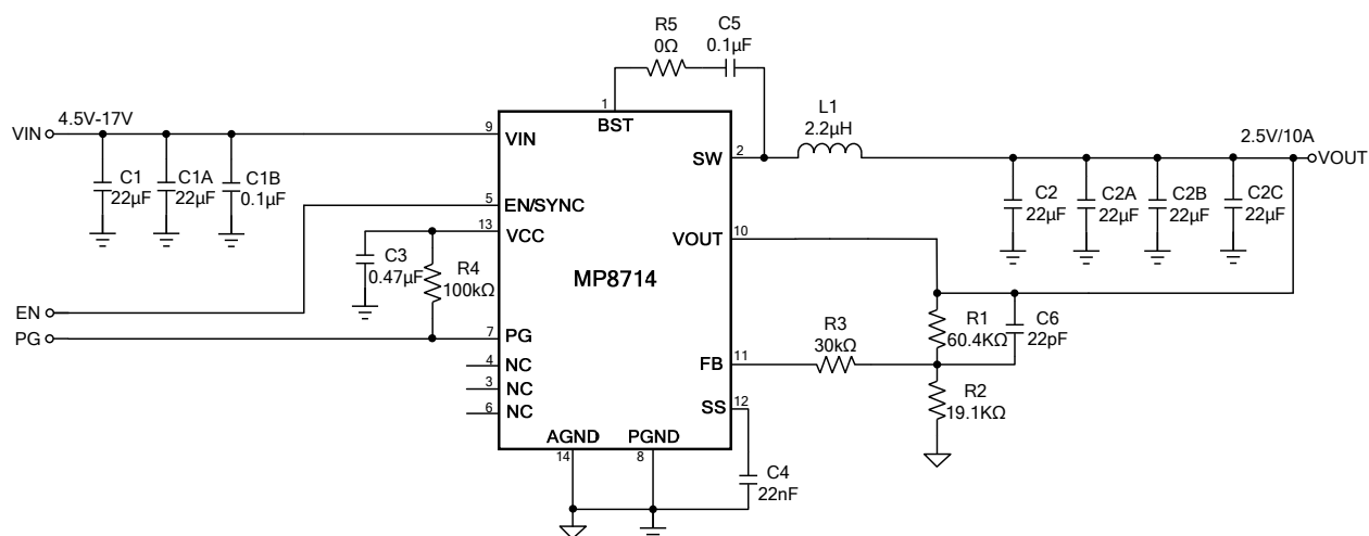
Figure 11: VIN = 4.5 - 17V, VOUT = 2.5V, IOUT = 10A
