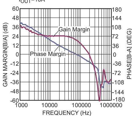
Bode Plot I_{OUT} = 10A
