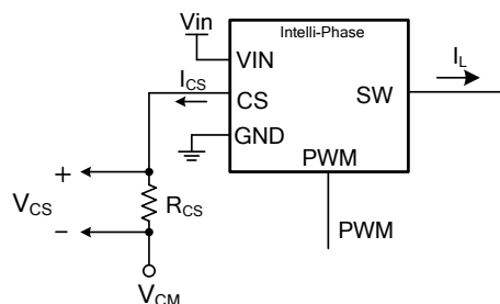
Fig.2 Typical Circuit Diagram for CS pin connection
