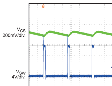
CS Output Waveform
