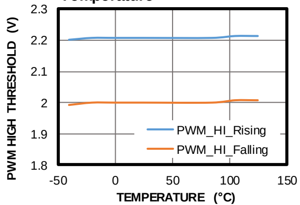
PWM High Threshold vs. Temperature
