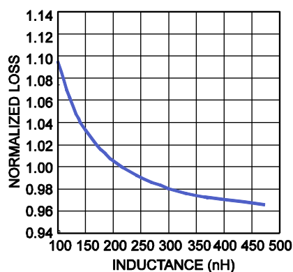
Normalized Power Loss vs. Inductance
