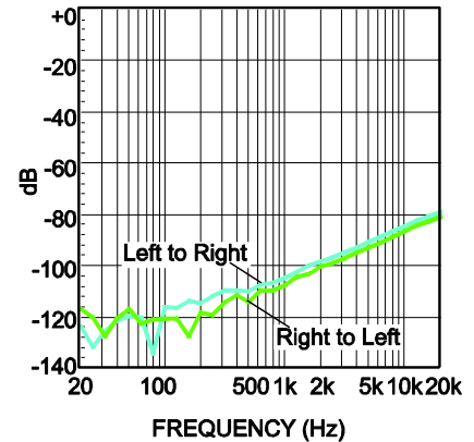
Cross Talk 18V, 8Ω + 66μH, P_{OUT} = 5W
