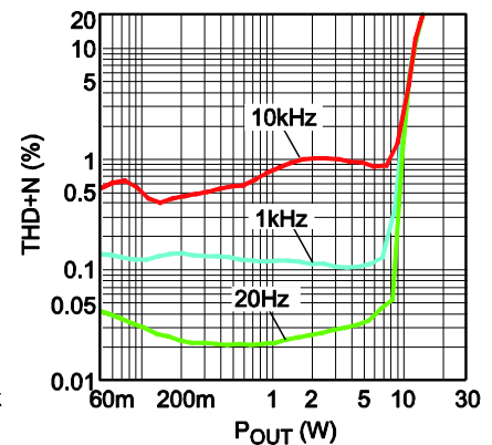
THD+N vs. P_OUT 12V, 6Ω + 44μH
