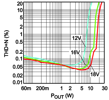
THD+N vs. P OUT 1kHz, 8Ω + 66μH
