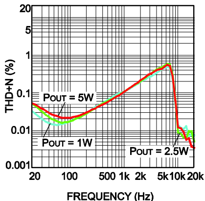
THD+N vs. Frequency 12V, 6Ω + 44μH
