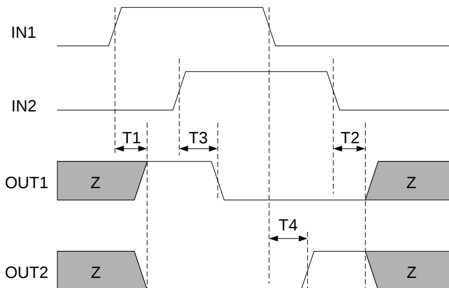
Figure 1: Input/Output Timing
