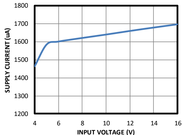
Supply Current vs. Input Voltage ON/PD = High
