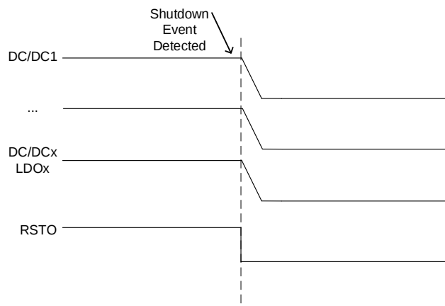
Figure 6: Shutdown Sequence
