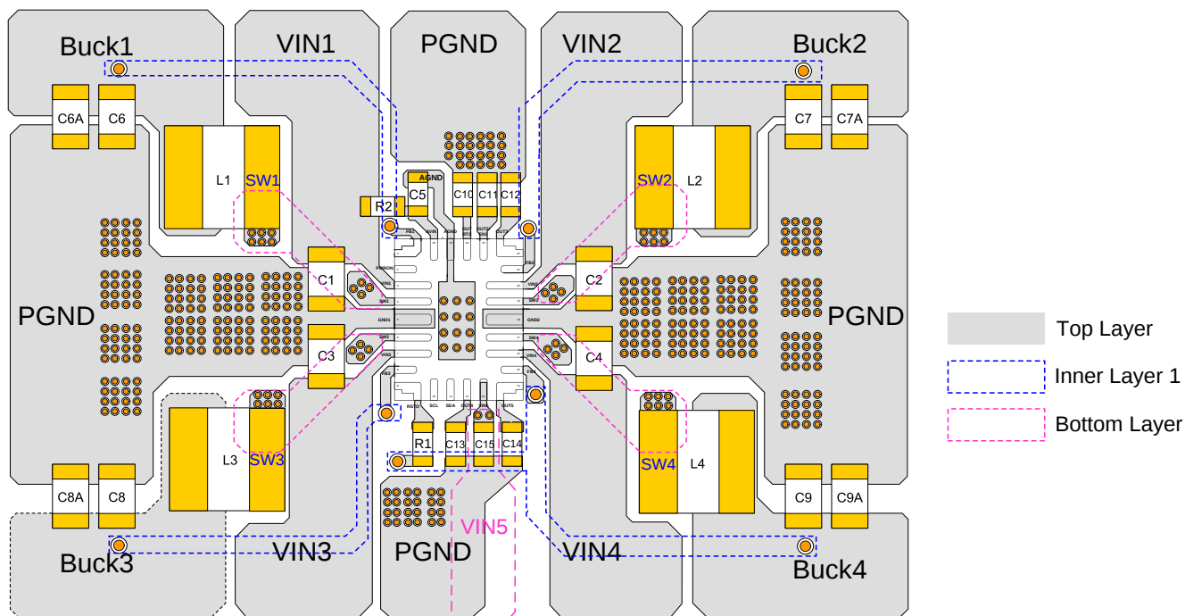
Figure 16: Recommended PCB Layout (21)
