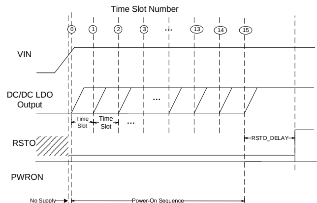
Figure 4: Power-On Sequence
