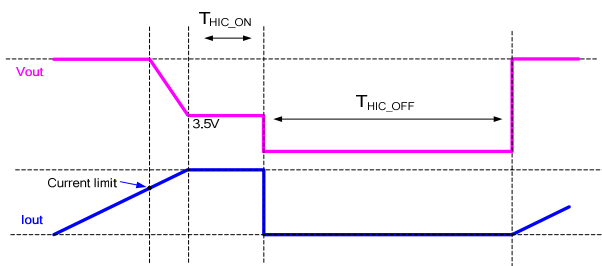
Figure 6: Over-Current Protection
