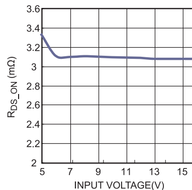
R DS_ON vs. Input Voltage I_{OUT}=1A
