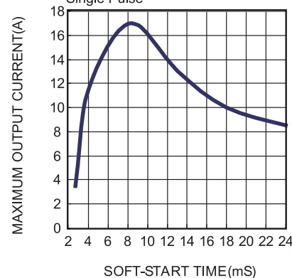
Maximum Output Current vs. Soft Start Time V_{IN}=12V , C_{OUT}=4700\mu F , En On, Single Pulse
