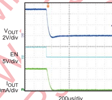
Turn Off Delay and Fall Time with 10uF Load R_{load}=5\Omega
