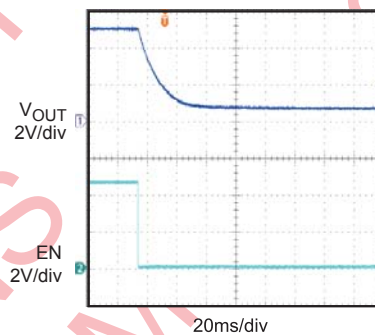
Turn Off Delay and Fall Time with 10uF Load C_{out}=10\mu F , no load
