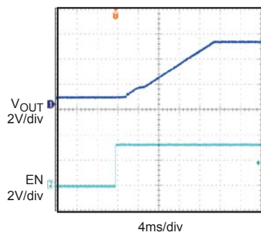
Turn On Delay and Rise Time with 1uF Load, 1nF Cdv/dt C_{out}=1\mu F , no load
