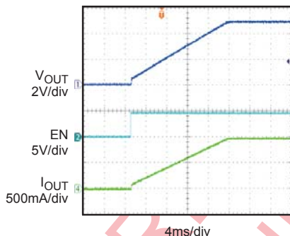
Turn On Delay and Rise Time with 10uF Load R_{load}=5\Omega
