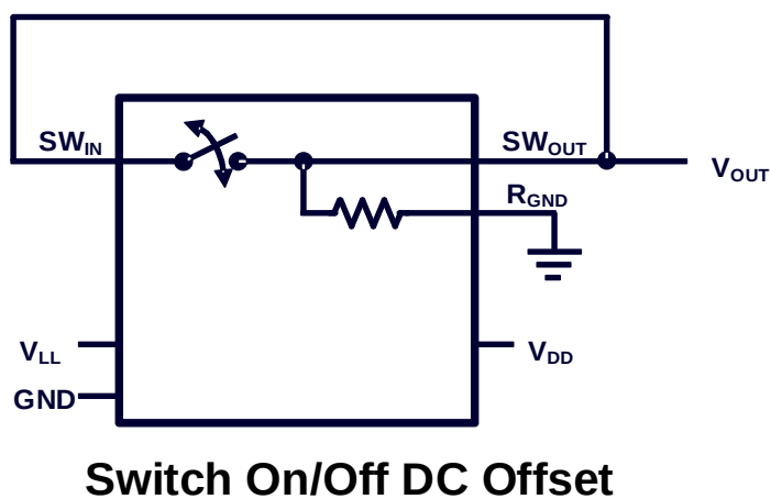
Figure 3: Test Circuit 3
