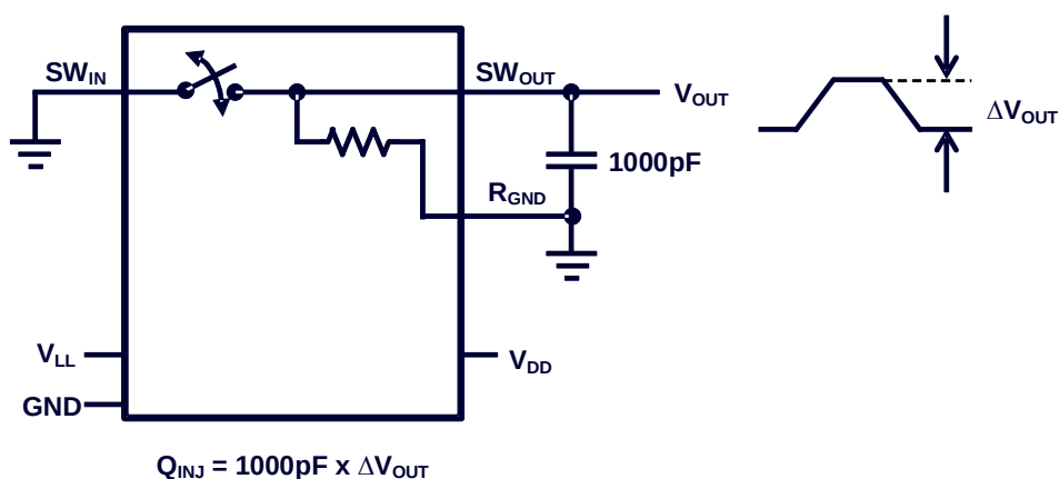
Figure 8: Test Circuit 8
