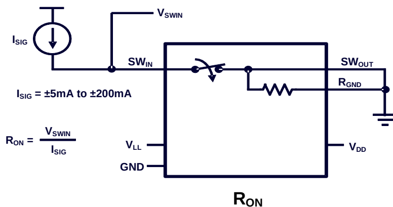
Figure 1: Test Circuit 1
