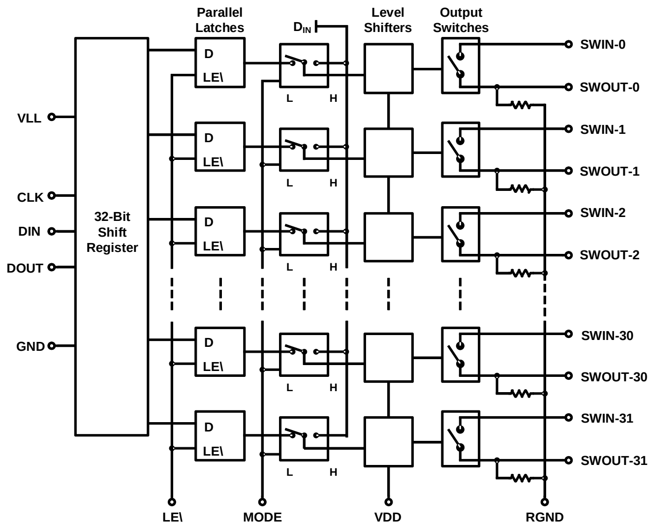
Figure 10: Functional Block Diagram
