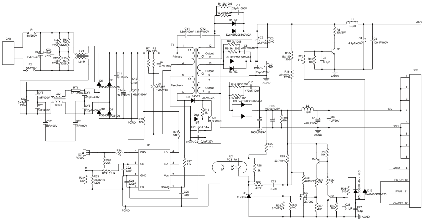
Figure 3: HFC0100 Flyback Schematic
