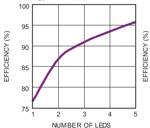
Efficiency vs. LED number
