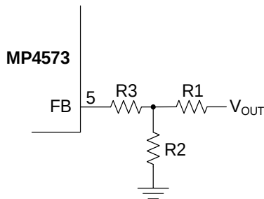
Figure 4: Feedback Network
