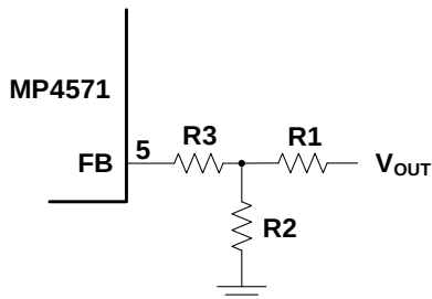
Figure 4: Feedback Network
