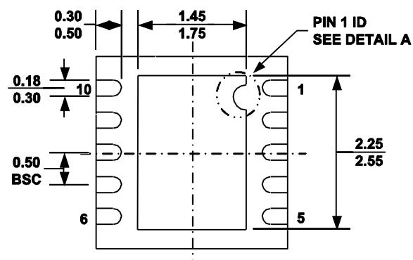
QFN10 (3x3mm)
