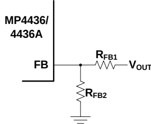
Figure 9: Feedback Network
