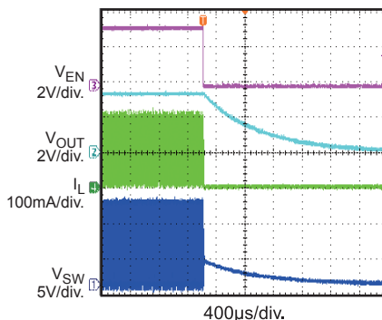
Shutdown Through EN I_{OUT} = 100mA
