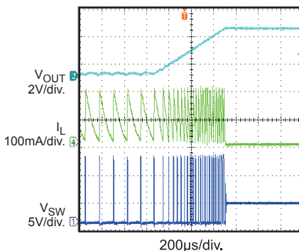
Short Circuit Recovery Short Circuit to I_{OUT} = 0
