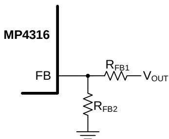
Figure 6: Feedback Network
