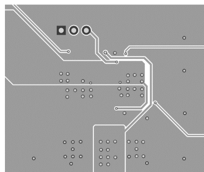
Mid-Layer 2
