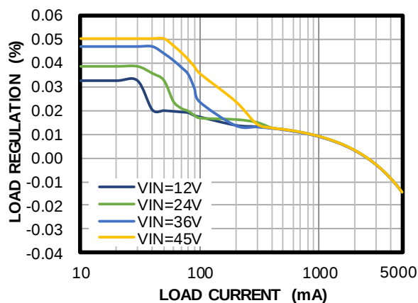
Load Regulation
