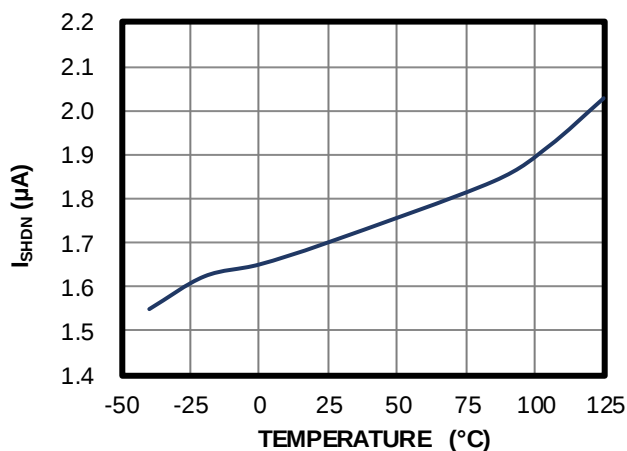
VIN Shutdown Current vs. Temperature
