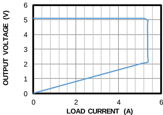
CC/CV Curve
