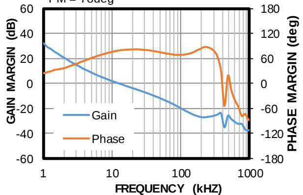
Bode Plot
