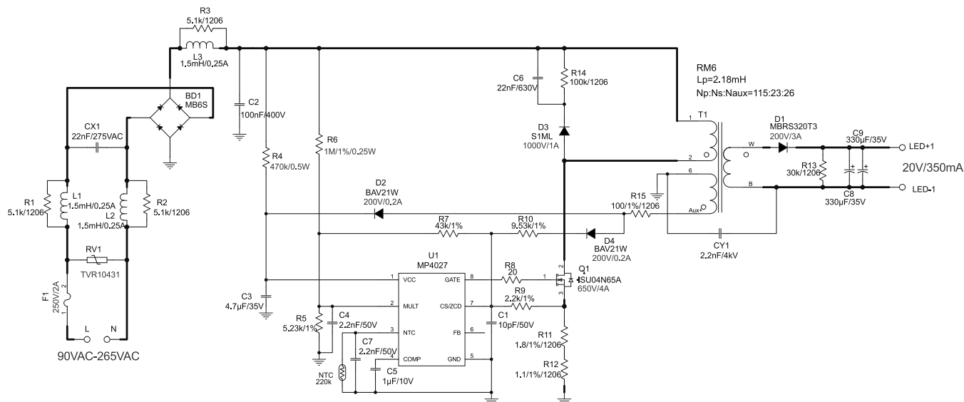
Figure 18: A19 Bulb Driver, 90-265VAC Input, Isolated Flyback Converter, V_O = 20V , I_{LED} = 350mA EVB Model: EV4027-J-00A
