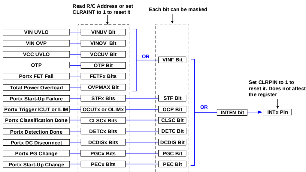
Figure 14: Interrupt Logic Diagram
