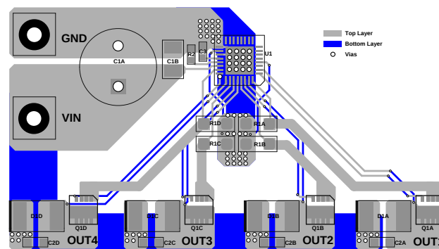
Figure 22: Recommended PCB Layout
