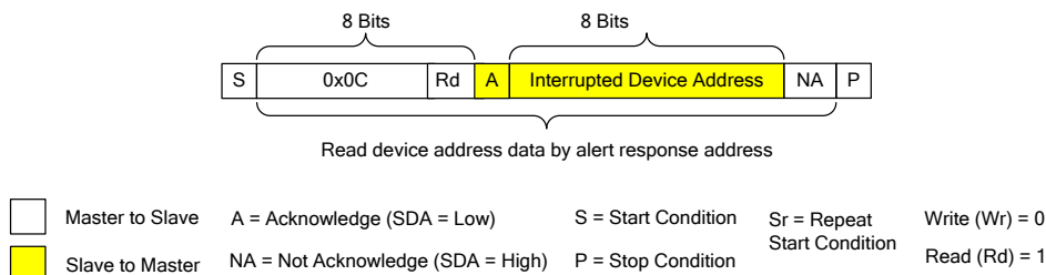
Figure 20: 0x0C Read Example
