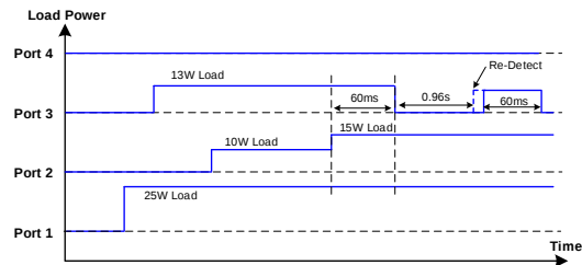
Figure 12: PMAX Power Management at 50W
