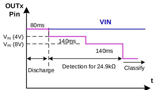
Figure 3: PD Detection Process
