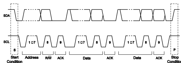
Figure 17: Complete Data Transfer
