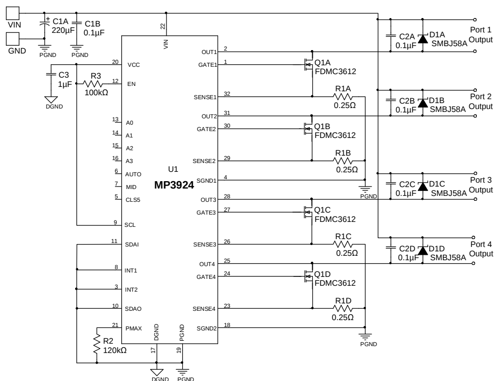
Figure 23: Typical Application Circuit without I 2 C Control
