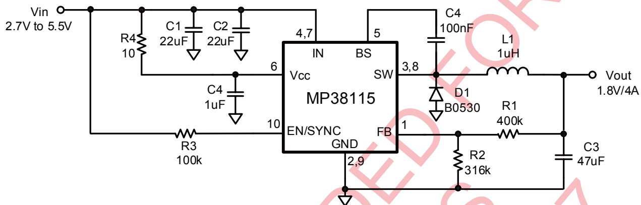
Figure3—Typical Application Circuit of MP38115
