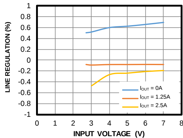
Line Regulation
