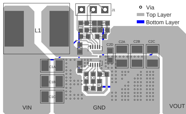
Figure 5: Layout Recommendation
