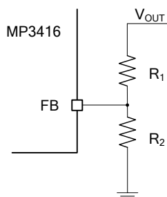
Figure 2: Feedback Network
