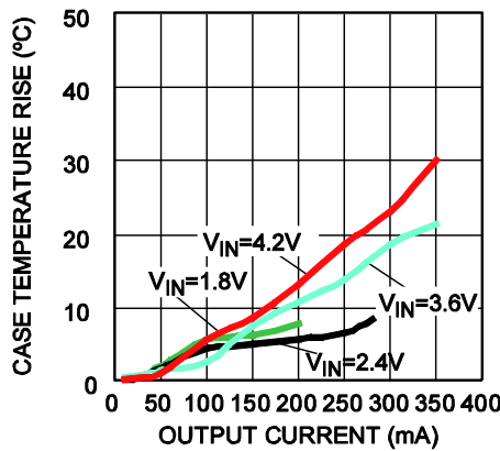
Case Temperature Rise vs. Output Current V_{OUT}=3.3V
