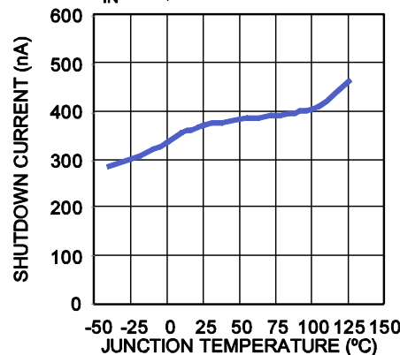
Shutdown Current vs. Junction Temperature V_{IN} = 1.8V , Enable = 0V
