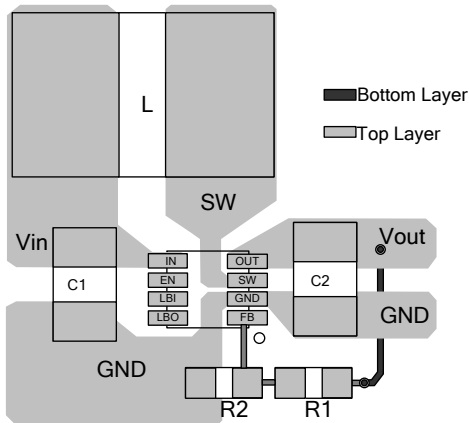
Figure 3: Recommended TSOT23 Layout
