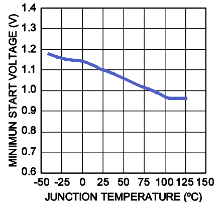
Minimum Start Voltage vs. Junction Temperature R_{load} = 1K\Omega
