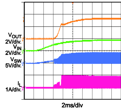
VIN Start-Up I_{OUT} = 0.2A
