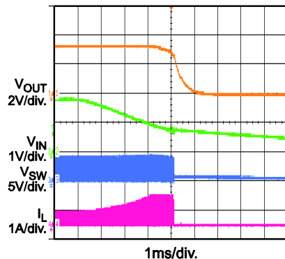
VIN Shutdown I_{OUT} = 0.2A
