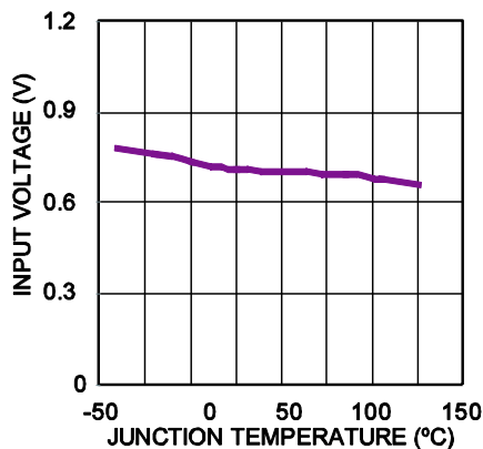
VIN Falling UVLO vs. Junction Temperature
