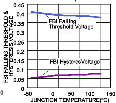
FBI Falling Threshold & Hysteresis Voltage vs. Junction Temperature
