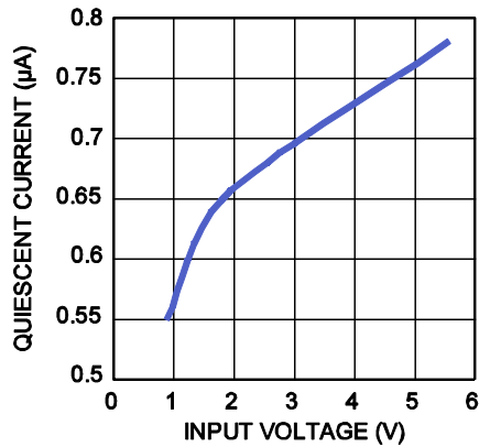
IN PIN Quiescent Current vs. Input Voltage V_{OUT} \geq V_{IN}
