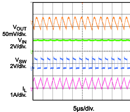
Output Ripple I_{OUT}=0.2A
