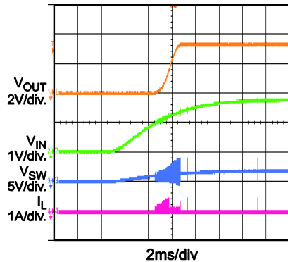
VIN Start-Up I_{OUT} = 0A
