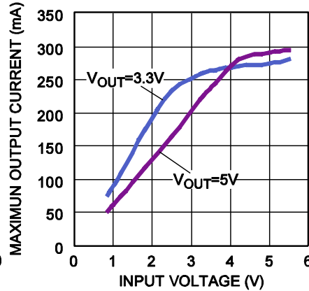
Maximum Output Current vs. Input Voltage (6)
