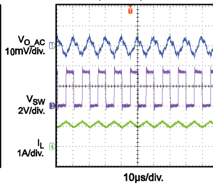
OUTPUT VOLTAGE RIPPLE (CCM)
