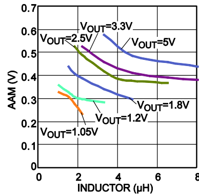
Figure 7—AAM selection for common output voltages ( V_{IN2} = 4.5 \text{ V} - 24 \text{ V} )
