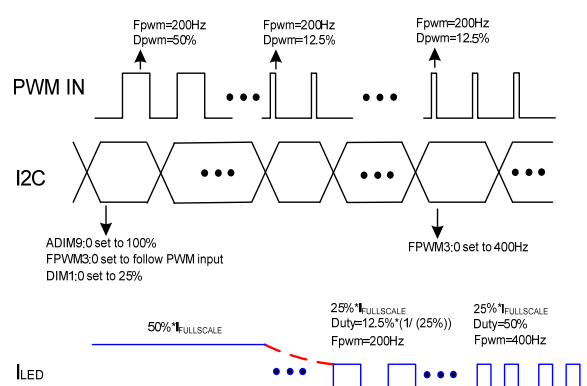
Figure 7: Mix Dimming from PWM Input
