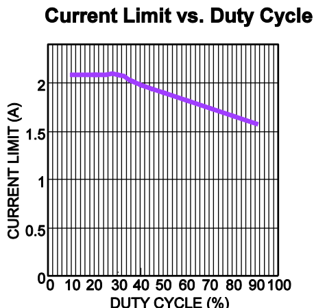
Figure 3—Current Limit Curve
