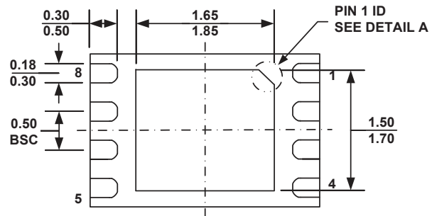
QFN8 (2mm x 3mm)
