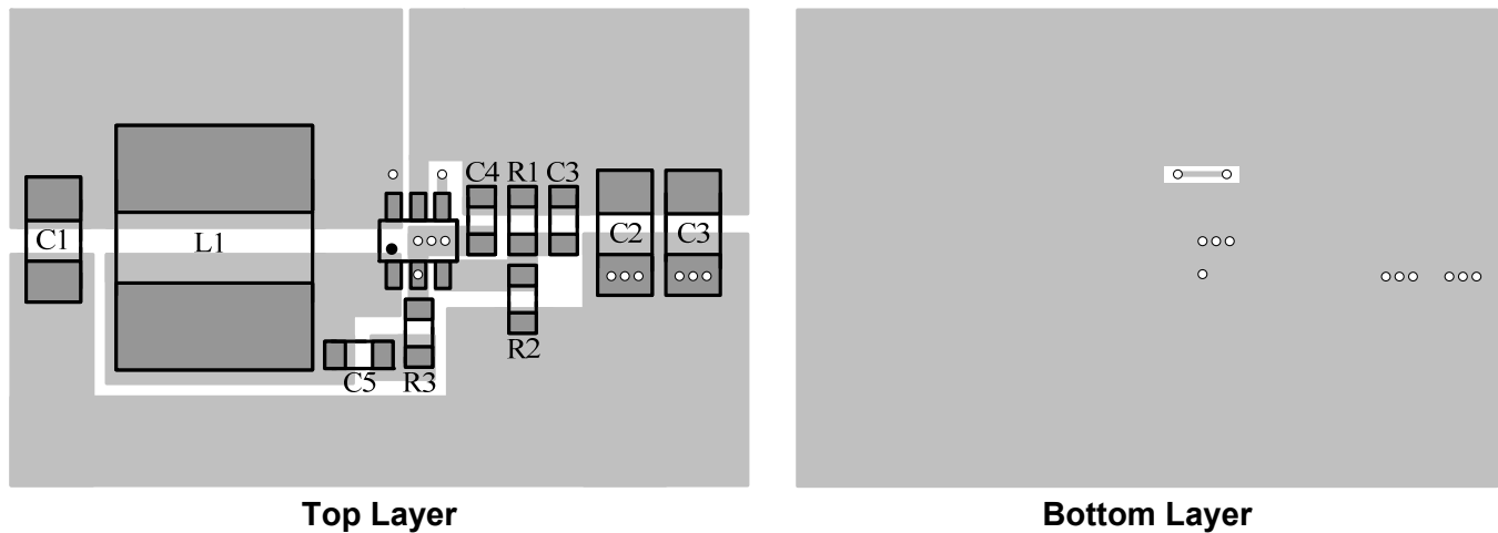
Figure3—PCB Layout
