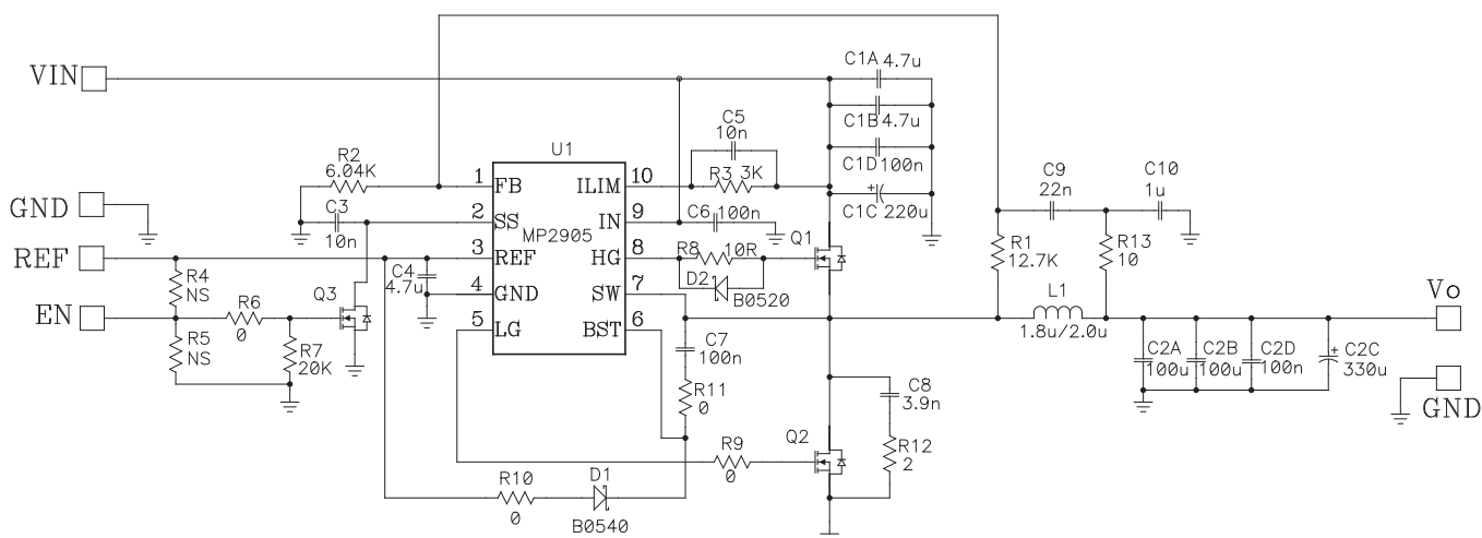
Figure 5—MP2905 Application Circuit
