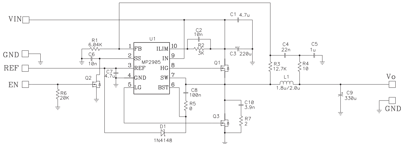
Figure 3—Typical Application Circuits for 12A Output
