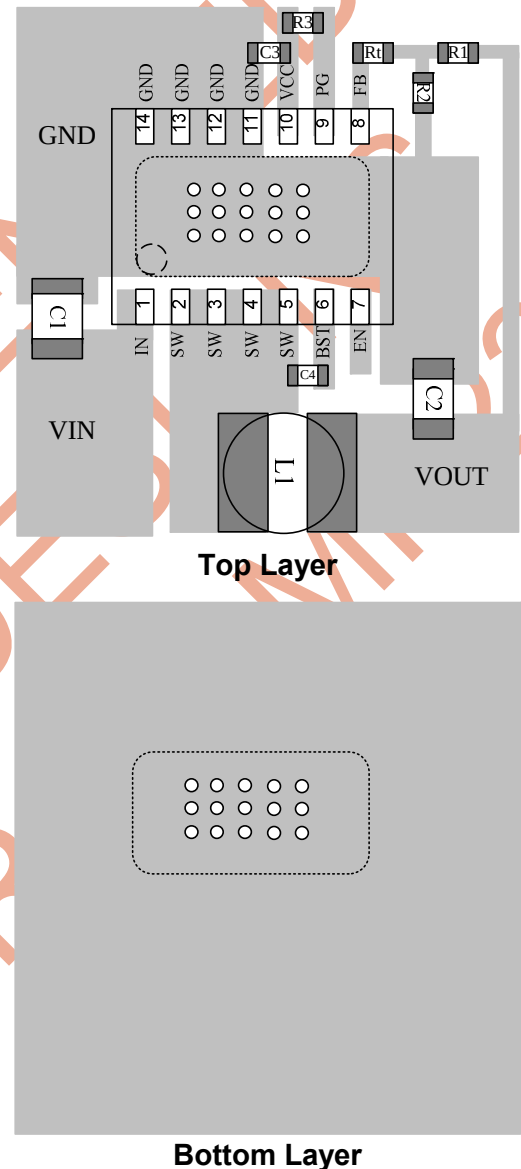
Figure 7—PCB Layout
