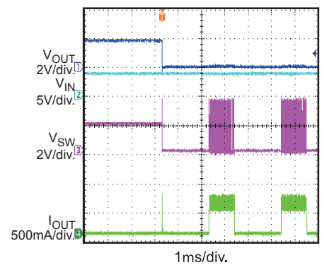
Short-Circuit Entry
