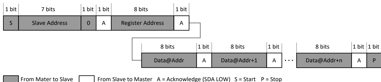
Figure 17: I²C Multi-Write
