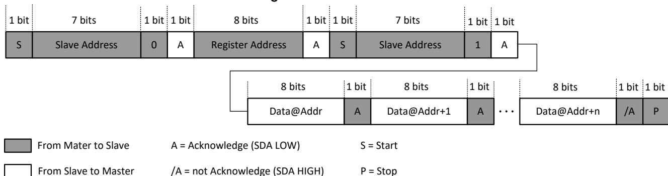
Figure 18: I²C Multi-Read
