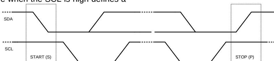
Figure 15: Start and Stop Conditions
