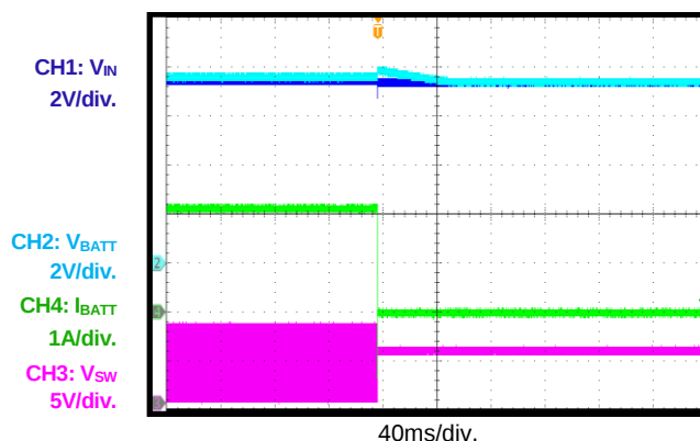
Boost Disabled
